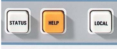
FIG 12: Online help
